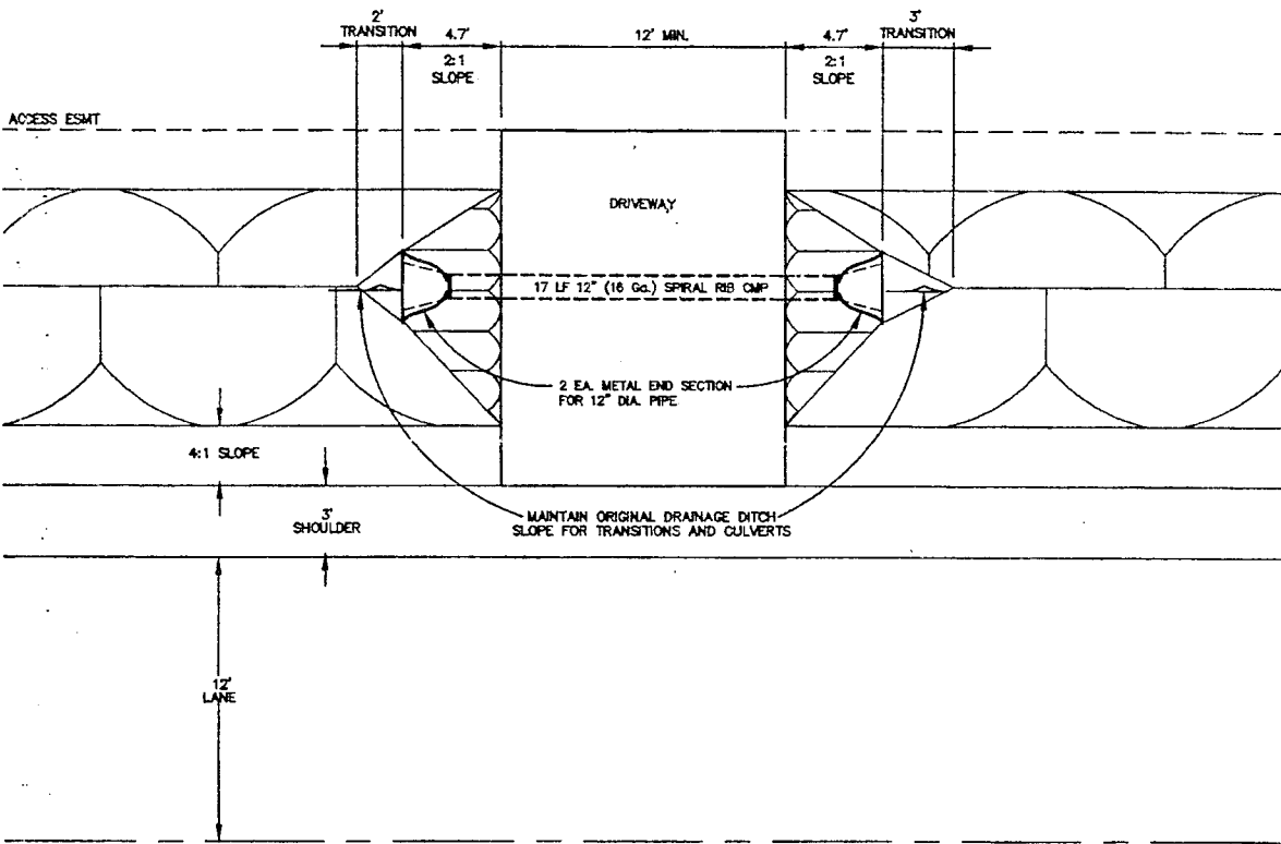
TYPICAL DRIVEWAY PLAN - UNPAVED SCALE: 1"=4'
