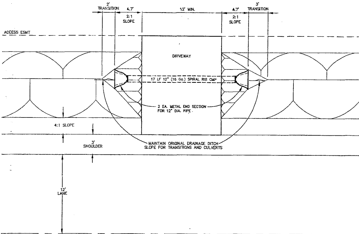
TYPICAL DRIVEWAY PLAN - PAVED SCALE: 1"=4'
