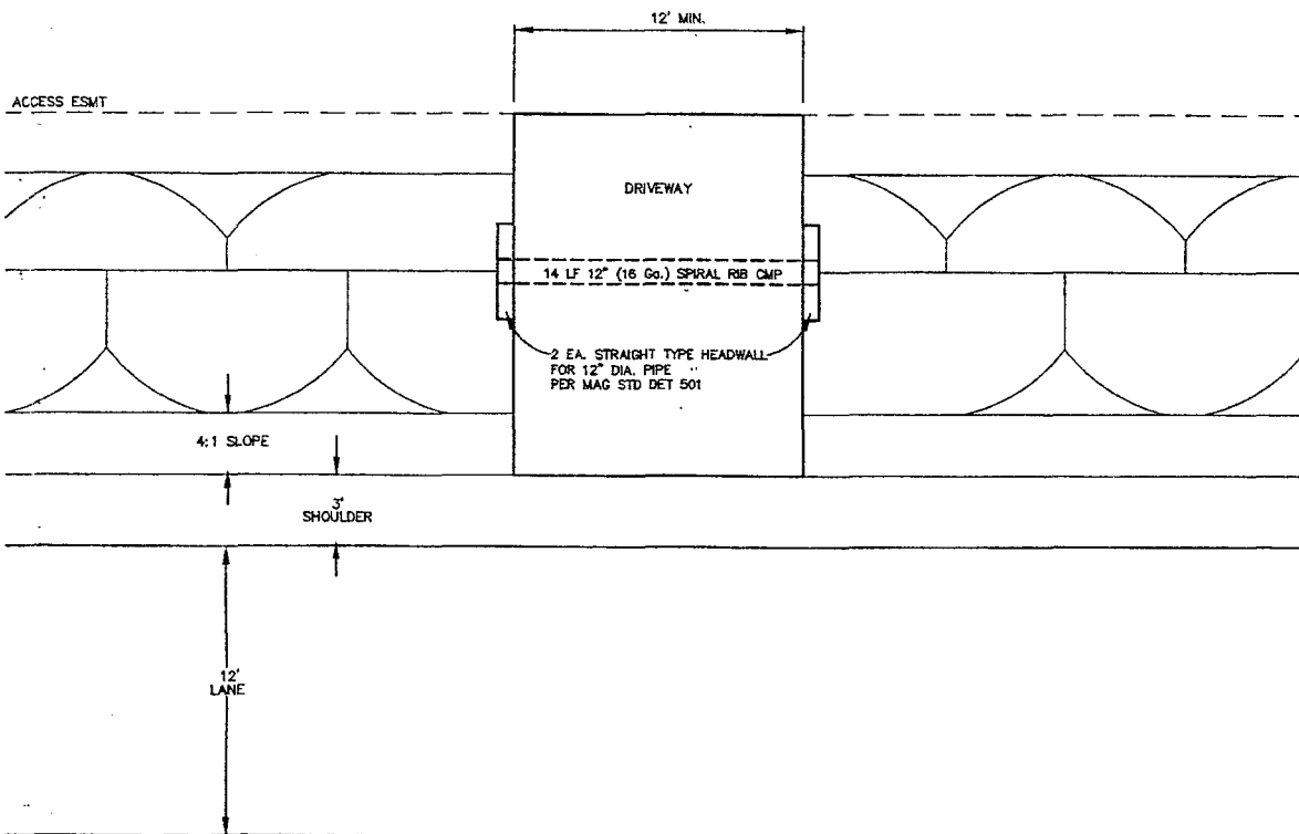
HEADWALL OPTION PLAN - PAVED SCALE: 1"=4'
