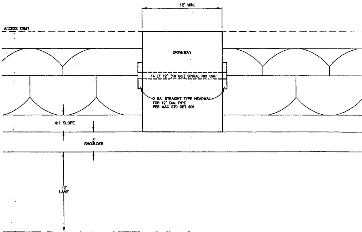
HEADWALL OPTION PLAN - UNPAVED SCALE: 1"=4'
